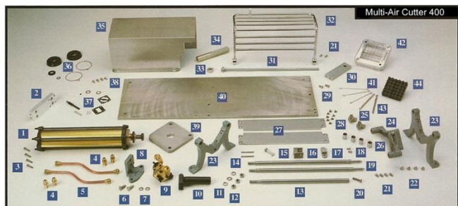
Parts for Multi-Purpose Air Cutter - 400 Series. Call for Quote
